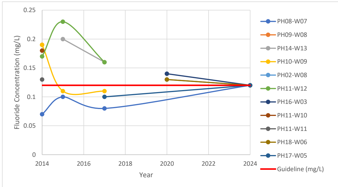
Figure 3-6 Fluoride in surface water measurements 1
